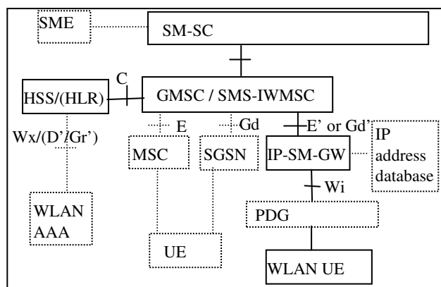
Figure 3 – Support of SMS over WLAN
